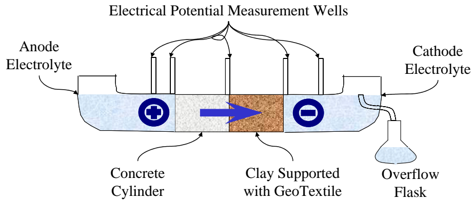
Figure 2. Cutaway view of experimental apparatus
